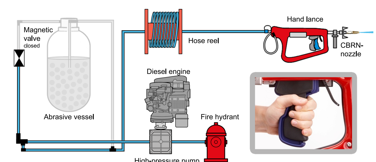
Water, CBRN nozzle
